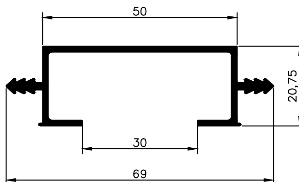
NX 1939 0,574 Kg/m
