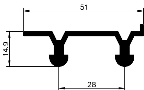
NX 1322 0,591 Kg/m
