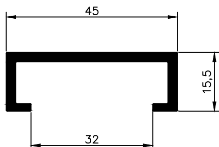
NX 1895 0,523 Kg/m
