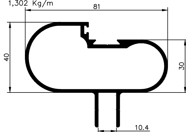
NX 4058 1,302 Kg/m
