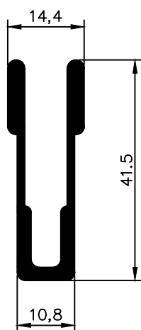
NX 0487 0,525 Kg/m
