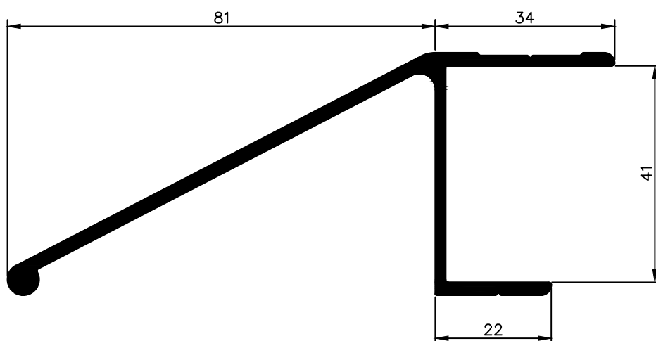
NX 4661 1,245 Kg/m
