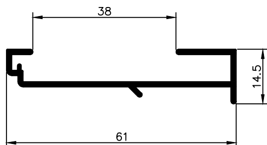
NX 0474 0,395 Kg/m
