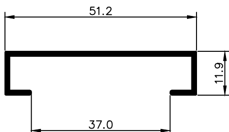
NX 0473 0,300 Kg/m
