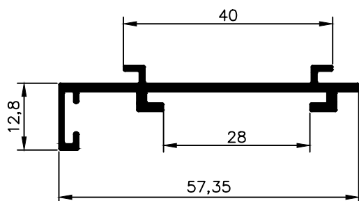
NX 4458 0,404 Kg/m
