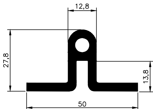
NX 1891 1,005 Kg/m
