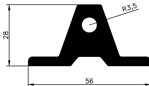
NX 3794 1,632 Kg/m
