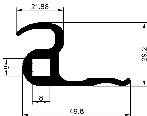
NX 1686 1,005 Kg/m
