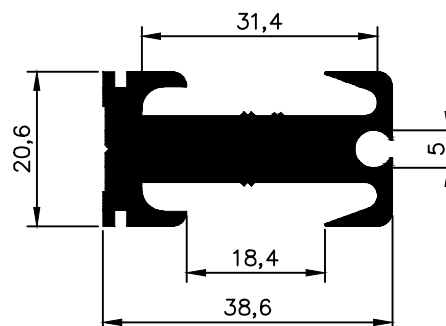
NX 1933 1,214Kg/m
