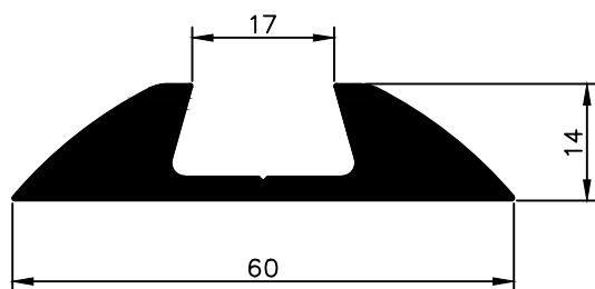
NX 5071 1,131 Kg/m
