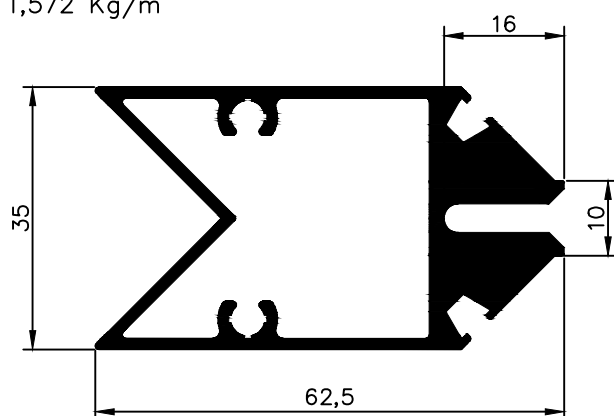
NX 2329 1,572 Kg/m
